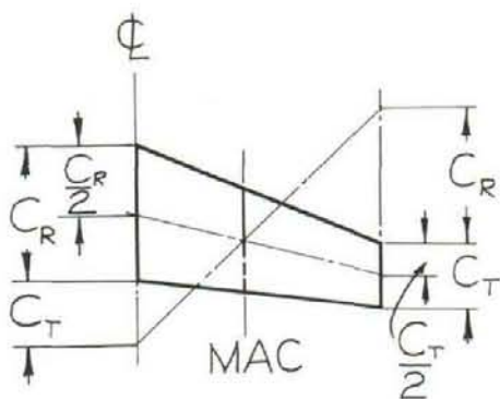
Fig. 4 — Graphical construction for approximate Mean Aerodynamic Chord (MAC)
