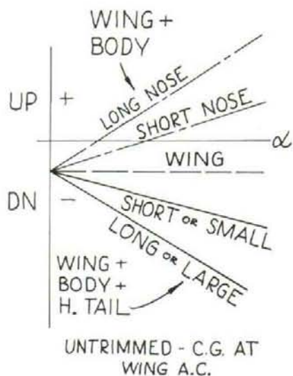
Fig. 8 — Effects of body nose length and tail length and size, c.g. at a.c.
