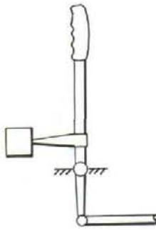
Fig. 16 — Bobweight schematic. This one requires increased pull if airplane accelerates upward (eyeballs down)
