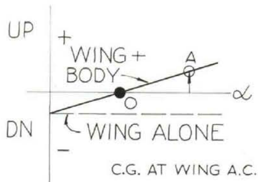
Fig. 7 — Effect of adding body
