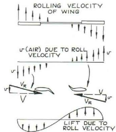
Fig. 18 — Effect of rolling velocity on wing lift
