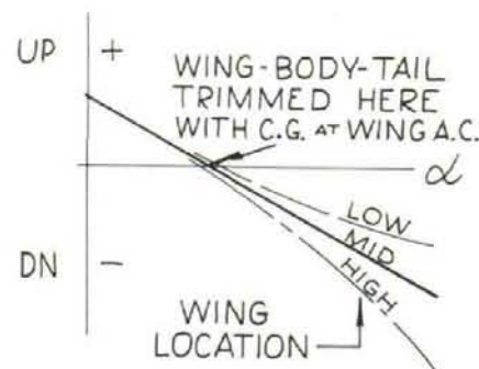
Fig. 10 — Effect of vertical movement of center of gravity
