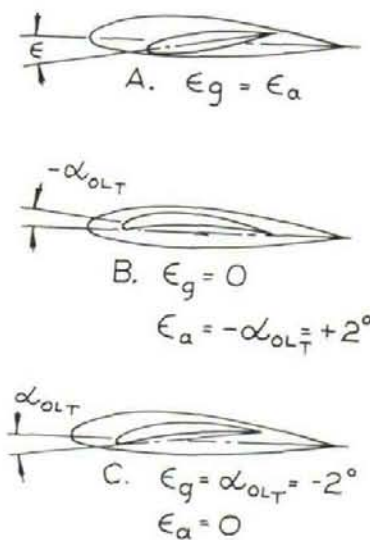
Fig. 22 — Geometric and aerodynamic twist. Subscript T refers to tip airfoil section. (A) equally cambered root and tip, (B) and (C) tip camber larger than root camber
