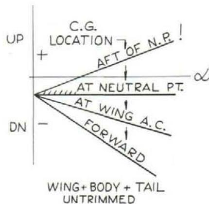
Fig. 9 — Effect of fore-and-aft movement of center of gravity
