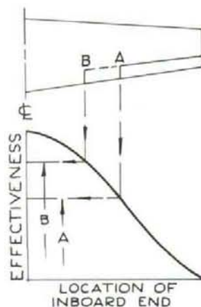
Fig. 19 — Aileron effectiveness gain due to aileron span increase
